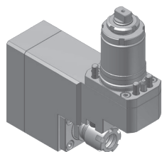
TSS861000 Slotting(Cross drilling/milling) unit
