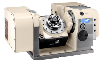
5 th AXIS TILTING RTT-111, CA
