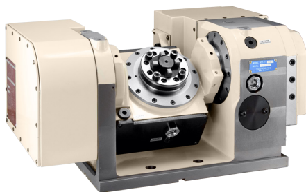
5 TH AXIS TILTING SERIES RTT-111, CA
