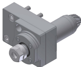
CTM3204161100-1 Cross drilling/milling unit
